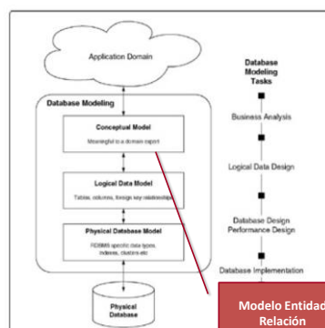
Figure 1-1: Database modeling in context. Ref. Database Modeling – T. Halpin EBD2014_1 - Mg. Mercedes Vitturini
