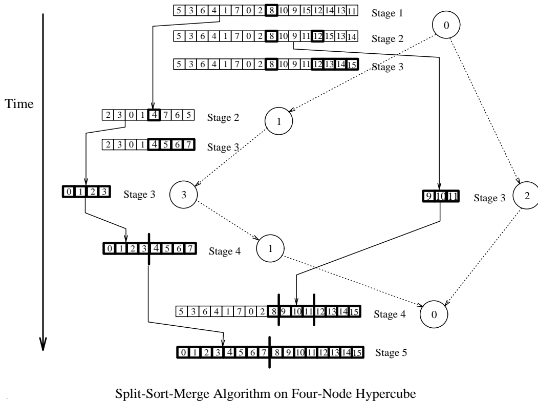
Figure 4.3 Tree-computation example
