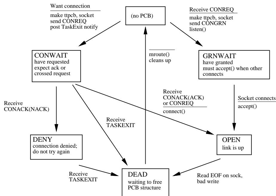
Figure 7.13 Task-task connection state diagram
