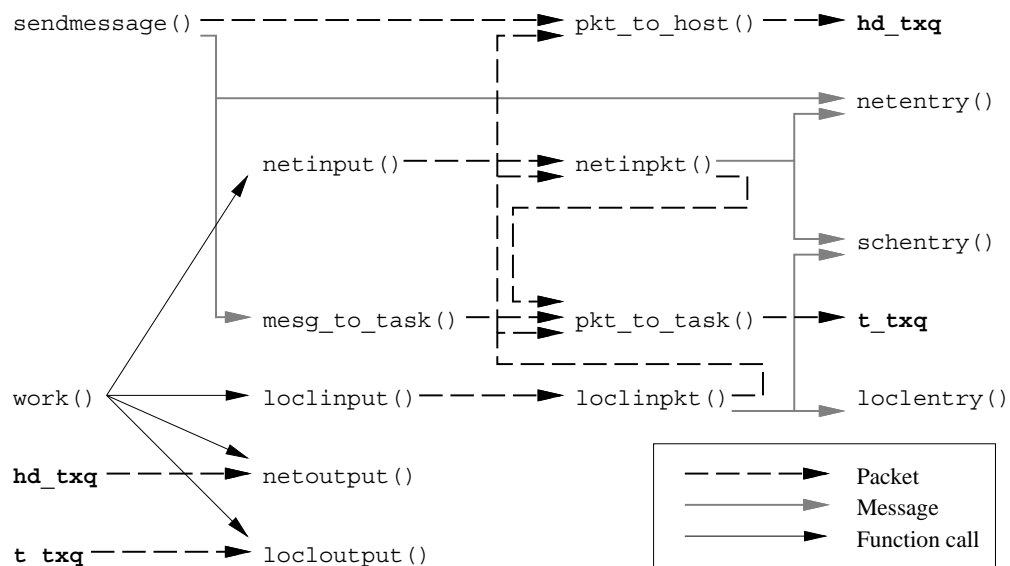
Figure 7.12 Packet and message routing in pvmd
