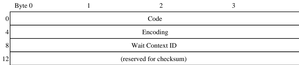
Figure 7.8 Message header
