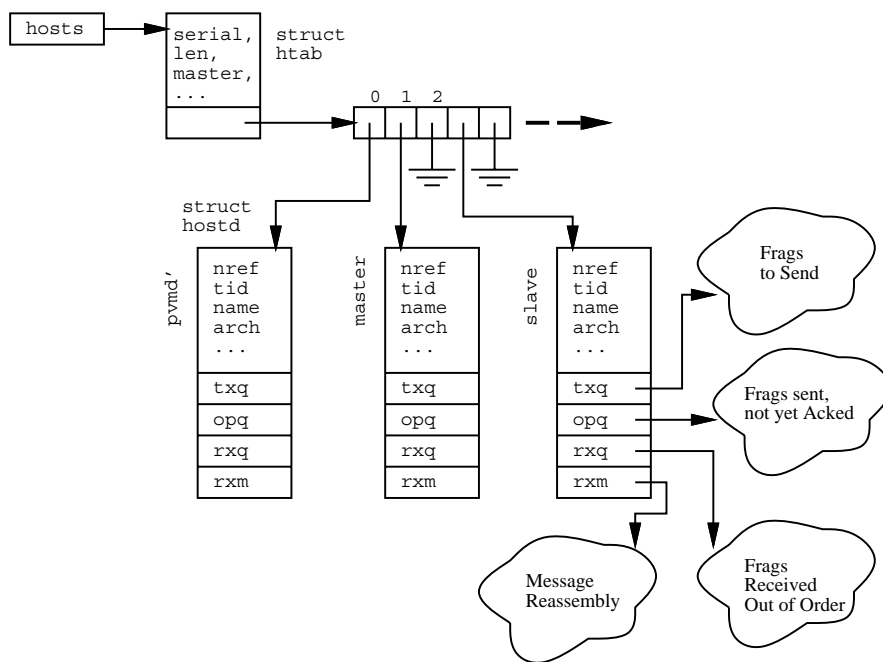
Figure 7.4 Host table
