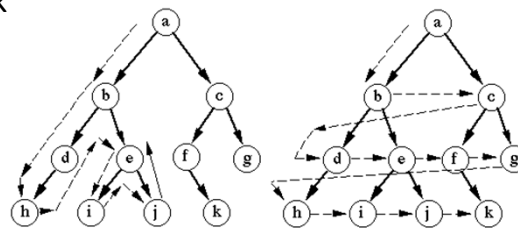
Depth-first search
