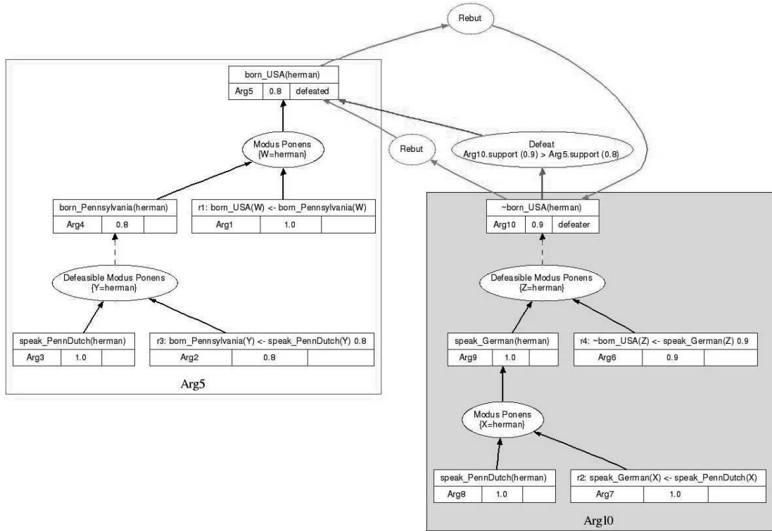
Figure 8 An example inference proof graph as generated by the ASPIC inference prototype. The proof graph is produced after reasoning over the claim ‘is Herman born in the USA?’. In this instance, using logical contradiction and defeat based on weakest link argument valuation, the claim is deemed inadmissible
