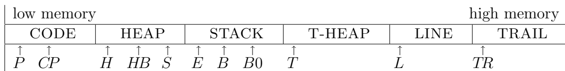
Figure 2: JAM memory architecture
