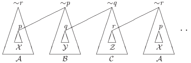
Fig. 8. Contradictory argumentation line
