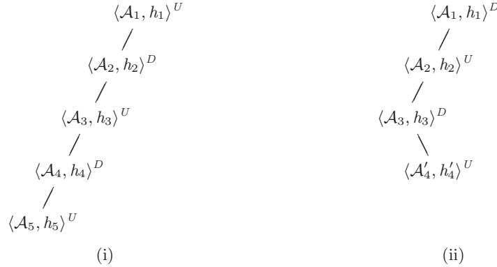
Fig. 12. Argumentation lines of Example 5.7
